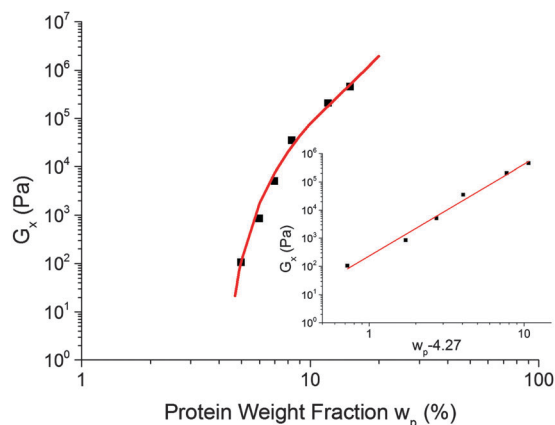
Fig. 10 The dependence of the cross-over modulus, G_\times on protein concentration, w , at the standard oil fraction and a constant sugar: water ratio of 2.9. The error bars for these data points are the size of the points or lower. The red curve is a fit to G_\times \sim \mathcal{G}(w - w_c)^f , eqn (6), with \mathcal{G} = 318 Pa, w_c = 4.27\% and f = 3.17 . The inset shows the same data and fitting in a plot against \log(w_p - 4.27\%) .
