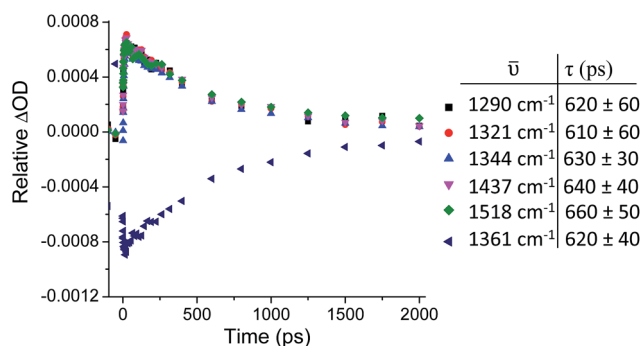
Fig. 5 ps-TRIR ( \lambda_{\text{ex}} = 400 nm) decay kinetics of the transient bands at 1290, 1321, 1344, 1437 and 1518 cm -1 and bleach at 1361 cm -1 of 1·2C1 (500 \mu\text{M} ) in D 2 O.
