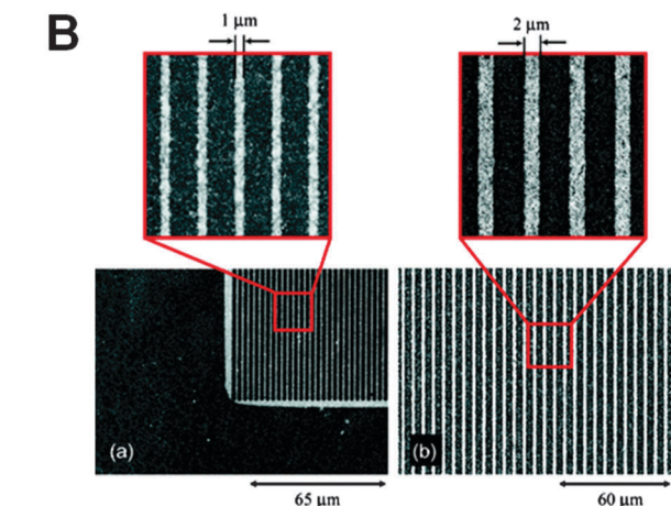
Fig. 6 (A) Scheme of the selective activation approach using patterned polyelectrolyte brushes and (B) SEM images of Cu patterns fabricated using the same method. Reprinted with permission from Azzaroni et al. 72 Copyright (2006) American Chemical Society.
