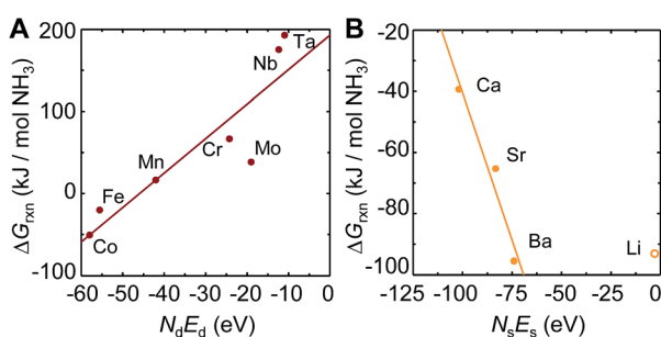
Fig. 2 Scaling of the free energy of the NH 3 evolution at 25 °C (computed from tabulated free energy data as described in Section 3.1) via metal nitride (A) reduction and (B) hydrogenation with the product of the number of electrons in the metal ground state, N , and the energy of these electrons, E , in the (A) d-states and (B) s-states. The metal marks the metallic constituent of the composition given with ESI.† Solid lines are fits to the data shown with solid symbols.
