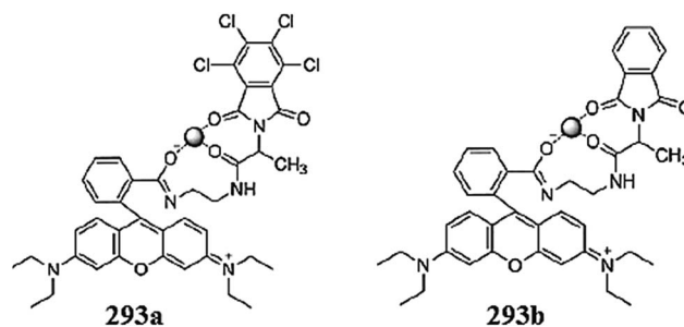
Fig. 257 Chemical structure of the ligand–Hg 2+ complexes.
