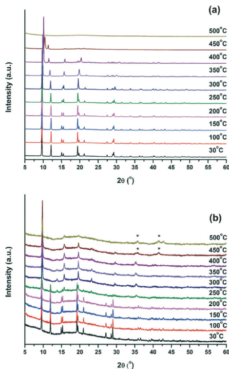
Fig. 5 VT-XPDP measurement of Ga-CFA-6 (a) and Fe-CFA-6 (b) from room temperature to 500 °C. Temperature steps of 50 °C were applied. (*) Peaks corresponding to the FeO phase (PDF no. 74-1886).
