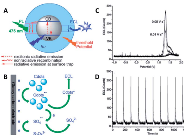
Fig. 15 (A) Schematic illustration of the PL and ECL emissions of CQDs. (B) The mechanism of ECL in the o-CQDs/ K_2S_2O_8 system. (C) ECL profiles of o-CQDs at a scan rate of 0.01 and 0.05 V s -1 . (D) The reproducibility of ECL in a continuous scan mode. Adapted with permission. 78 Copyright 2013, Wiley-VCH.
