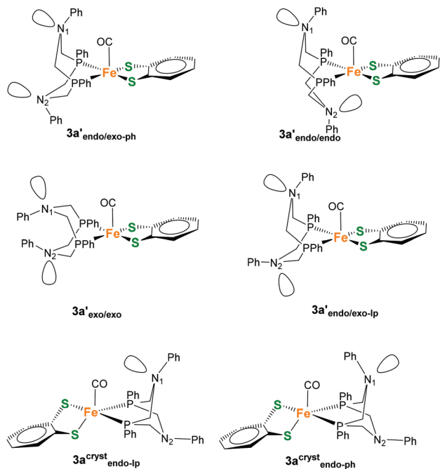
Fig. 8 Potential coordination isomers 3a' and 3a'^{\text{crist}} with different exo/endo conformations of the 6-membered FePCNCP heterocycles as well as different orientations of the N-Ph substituent.
