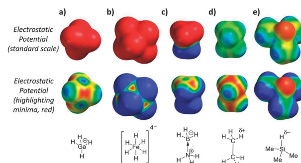
Fig. 2 Electrostatic surface potentials (ESPs) of representative dihydrogen acceptors. Electrostatic potentials on the top row are scaled using a standard scale from -50 \text{ kJ mol}^{-1} (red) to +50 \text{ kJ mol}^{-1} (blue), while those on the bottom row are scaled to highlight the ESP minimum (ESP min , red) to ESP min + 50 \text{ kJ mol}^{-1} (blue). Minimised geometries and ESPs were calculated using B3LYP/LACVP.
