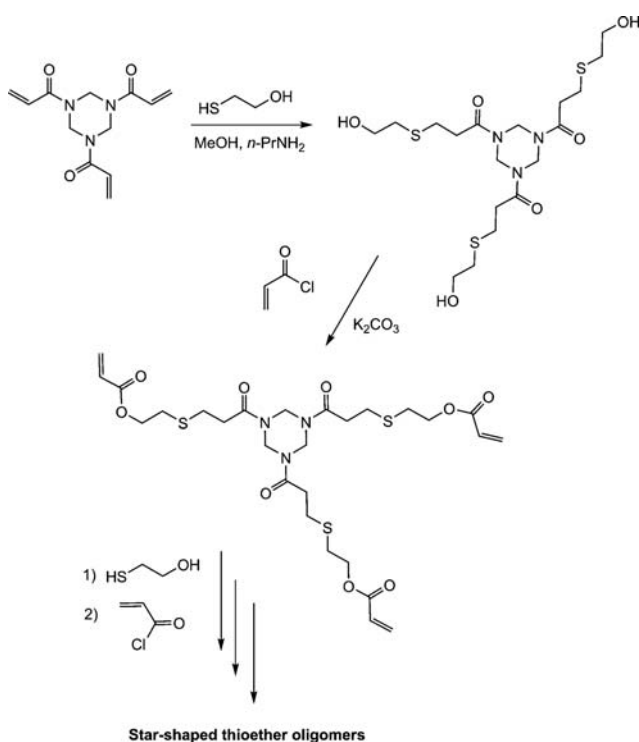
Scheme 21 Synthesis route to 3-arm star thioether oligomers via sequential thiol-ene/acetylation reactions.
