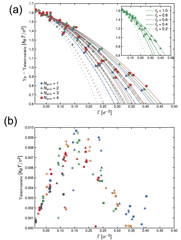
Fig. 4 Dependence of \gamma_p - \gamma_{electrostatic} with surface concentration of the active component, \Gamma , for different systems of stars with number of arms, N_{arm} , and degree-of-protonation f_q (a). Lines in (a) are fits to Eq. 4 and inset in (a) shows the system with N_{arm} = 3 . Solid, long-dashed, dotted, short-dashed and loosely-dotted lines pertains to f_q of 1.0, 0.8, 0.6, 0.4 and 0.2, respectively. The electrostatic component of interfacial tension, \gamma_{electrostatic} , is given by Eq. 7. The symbols in (b), \bullet , + , \blacktriangle and \blacksquare pertains to systems with N_{arm} of 1, 2, 3 and 4, respectively. The colors of the symbols in (b): blue, orange, green, red and gray pertains to f_q of 1.0, 0.8, 0.6, 0.4 and 0.2, respectively.
