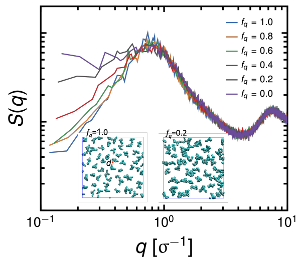
Fig. 8 Scattering of the in-plane structure of PS of the system with N_{arm} = 3 , \phi_s = 0.18 and initially dissolved in 2 \times 10^4 oil beads at different values of f_q . Insets are representative snapshots where d is the characteristic distance between PS domains.
