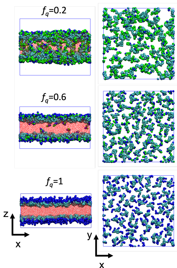
Fig. 7 Side view (left panels) and top view (right panels) of the system with N_{arm} = 3 , \phi_s = 0.18 and initially dissolved in 2 \times 10^4 oil beads at different values of f_q . Cyan beads represent PS, blue beads represent QP2VP, green beads represent un-protonated P2VP (IP2VP) and red dots represent oil beads. The solvent beads are not shown for clarity. The top view images show only the top-most interface with solvent and oil beads not shown for clarity.
