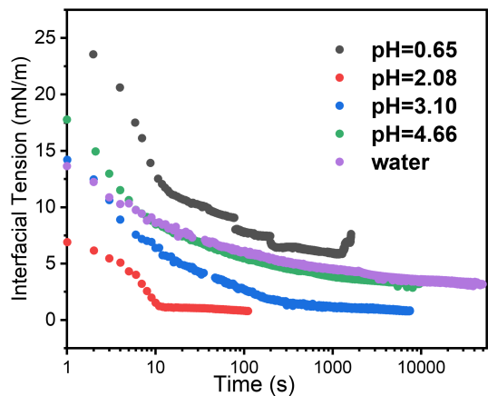
Fig. 9 Time-dependent interfacial tension of toluene dissolved 4-arm star block copolymer against the water phase with variation of pH. 4-arm star block copolymer: 0.1 mg/ml, where PS core and P2VP corona has MW 2800 g/mol and 4200 g/mol per arm, respectively. The pH was adjusted by addition of HCl.
