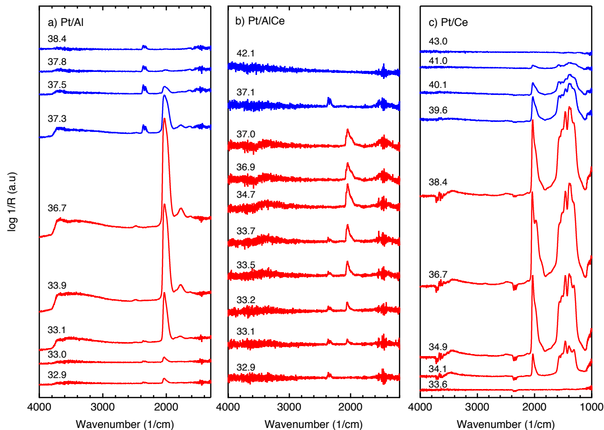
Fig. 5 Evolution of IR bands in the wavenumber region 1000\text{--}4000\text{ cm}^{-1} for (a) Pt/Al, (b) Pt/AlCe and (c) Pt/Ce catalysts exposed to 0.1% methane while changing the oxygen concentration from 3000 ppm ( S=1.5 ) to 0% ( S=0 ) (red lines) and then back to 3000 ppm (blue lines) at an inlet gas temperature of 400^\circ\text{C} . The insert numbers indicate the time (min) in the dynamic experiment where the spectra were recorded.
