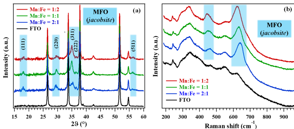
Fig. 2 (a) XRD patterns and (b) Raman spectra for MFO specimens grown on FTO from different mixtures of \text{Mn}(\text{hfa})_2\cdot\text{TMEDA} and \text{Fe}(\text{hfa})_2\cdot\text{TMEDA} precursors. Curves have been vertically shifted for clarity. The XRD pattern and Raman spectrum of the bare FTO substrate are also reported for comparison. In both panels, the main signals from the MFO spinel phase are highlighted by a pale blue background.
