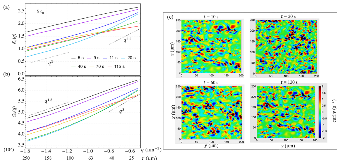
Fig. 10 (a) Kinetic energy spectrum K_s(q) (units (\mu\text{m s}^{-2})^2 ) and (b) enstrophy spectrum \Omega_s(q) (units \text{s}^{-2} ) as a function of the wave vector q ( \mu\text{m}^{-1} ) at different times for 5c_0 . The spectra K_s(q) and \Omega_s(q) are averaged over 5 consecutive frames (or 1 s). (c) Vorticity curl \mathbf{v} for 5c_0 at different times.
