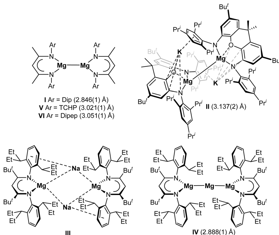
Fig. 1 Previously reported examples of magnesium(i) and magnesium(0) compounds (Mg–Mg bond lengths in parentheses). Dip = 2,6-diisopropylphenyl, TCHP = 2,4,6-tricyclohexylphenyl, Dipec = 2,6-di(3-pentyl)phenyl.
