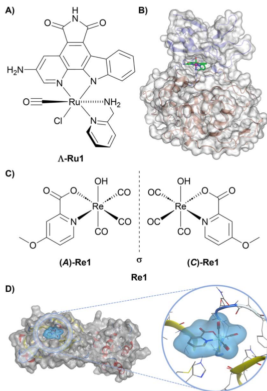
Fig. 2 Representative metal complexes as protein inhibitors. (A) Chemical structure of \Lambda -Ru1. (B) Crystal structure of GSK3 \beta with \Lambda -Ru1 bound to the ATP-binding (PDB: 1Q3D). Reprinted with permission from ref. 98 (L. Feng et al. , 2011), Copyright 2011 American Chemical Society. (C) Chemical structure of the racemic mixture of Re1 , showing the ( A )- Re1 and ( C )- Re1 enantiomers. (D) Computationally predicted binding pose of the Re1 fragment bound to the thiol group of Cys145 of 3CL PRO (PDB: 6Y2F). Reproduced from ref. 99 (J. Karges et al. , 2023), licensed under CC BY-NC 3.0.
