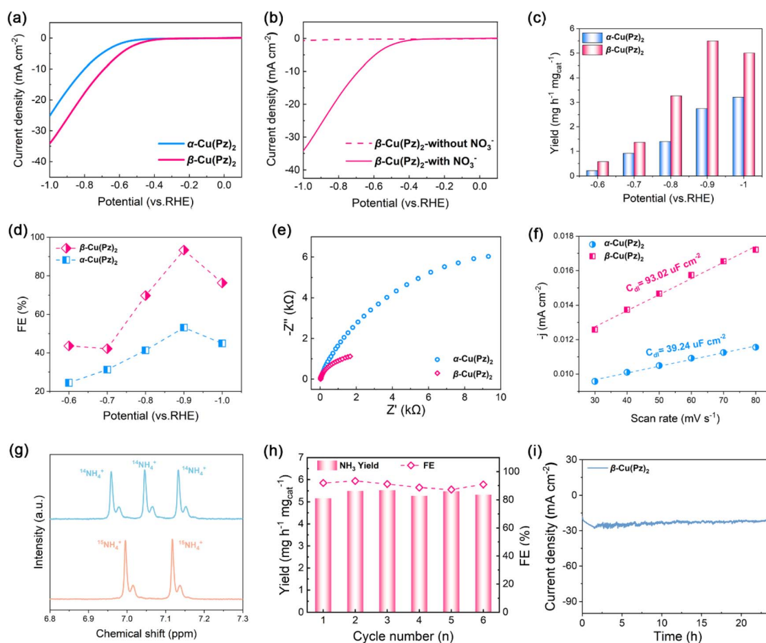
Fig. 3 (a) LSV curves for \alpha -Cu(Pz) 2 (blue) and \beta -Cu(Pz) 2 (pink) in the electrolyte. (b) Comparison of LSV curves for \beta -Cu(Pz) 2 recorded with (solid line) and without (dashed line) NO 3 - . (c and d) NH 3 yield rates and corresponding FEs of \alpha -Cu(Pz) 2 (blue) and \beta -Cu(Pz) 2 (pink) at different potentials. (e and f) EIS and ECSA measurements of the two samples. (g) 1 H NMR spectra of the products after NO 3 RR over \beta -Cu(Pz) 2 using K 14 NO 3 (blue) and K 15 NO 3 (orange) as the feeding nitrogen sources. (i) Cycling stability tests of \beta -Cu(Pz) 2 at -0.9 V (vs. RHE) for 6 cycles. (h) Time-dependent current density curve at -0.9 V (vs. RHE) for over 24 h for \beta -Cu(Pz) 2 .
