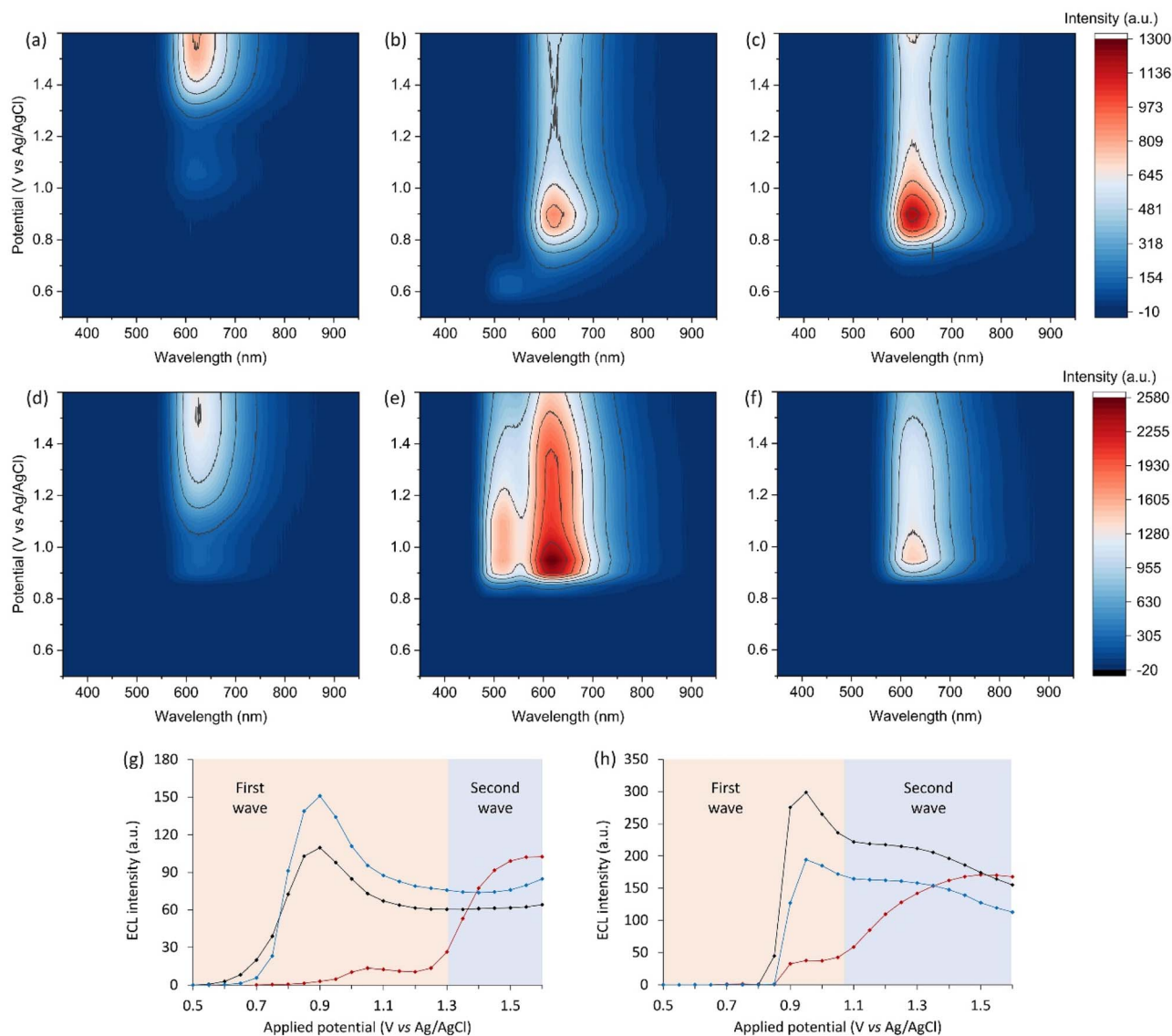
Fig. 3 (a–f) Contour plots of ECL intensity as a function of wavelength and applied potential, for: 10 μM [Ru(bpy) 3 ] 2+ with (a) no redox mediator, (b) 100 μM Ir(ppz) 3 , or (c) 100 μM Ir(ppz) 3 in acetonitrile with 10 mM TPrA and 0.1 M TBAPF 6 ; or 1 μM [Ru(bpy) 3 ] 2+ with (d) no redox mediator, (e) 100 μM [Ir(sppy) 3 ] 3- , or (f) 100 μM [Ir(sppz) 3 ] 3- in aqueous 'ProCell' solution containing 180 mM TPrA, 0.1% polidocanol surfactant, and 0.3 M phosphate buffer (pH 6.8). 8 (g and h) Comparisons of relative ECL intensity of [Ru(bpy) 3 ] 2+ (integrated spectral distribution) without a redox mediator (red plot) or (g) when using Ir(ppz) 3 (black plot) or Ir(ppz) 3 (blue plot) in acetonitrile; and (h) when using [Ir(sppy) 3 ] 3- (black plot) or [Ir(sppz) 3 ] 3- (blue plot) in aqueous media, extracted from the data shown in Fig. 3a–c and d–f, respectively. Data in Fig. 3d–f and h is from ref. 18. In the plots for Ir(ppz) 3 and [Ir(sppy) 3 ] 3- in Fig. 3g and h, respectively, the emission from [Ru(bpy) 3 ] 2+ has been deconvoluted from that of the redox mediator (Fig. S6 and S16). The coloured boxes in Fig. 3g and h show the potentials below (red) and above (blue) the E_{\text{ox}} of [Ru(bpy) 3 ] 2+ in that solvent.
