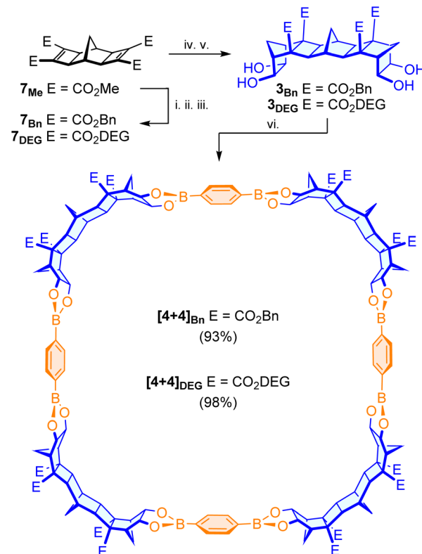
Scheme 3 Tuning of physical properties through ester modification. (i) KOH, \text{H}_2\text{O} : \text{THF} : \text{MeOH} (4 : 1 : 1), reflux, 24 h. (ii) \text{SOCl}_2 , \text{CHCl}_3 , reflux, 1.5 h. (iii) Benzyl alcohol or diethylene glycol monomethyl ether (4.5 eq.), \text{CHCl}_3 , reflux, 2 h. (iv) CPD (8 eq.), DMF, RT, 7 days. (v) \text{OsO}_4 (1 mol%), NMO (3.0 eq.), acetone: \text{H}_2\text{O} , RT, 3 days. (vi) \text{CHCl}_3 , 100 °C, 24 h.
