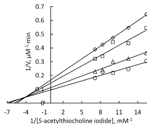
Fig. 2 Lineweaver–Burk plot for inhibition of AChE by compound 22. The concentrations of the inhibitor were 0 (○), 70 nM (Δ), 140 nM (□), and 280 nM (◇).
