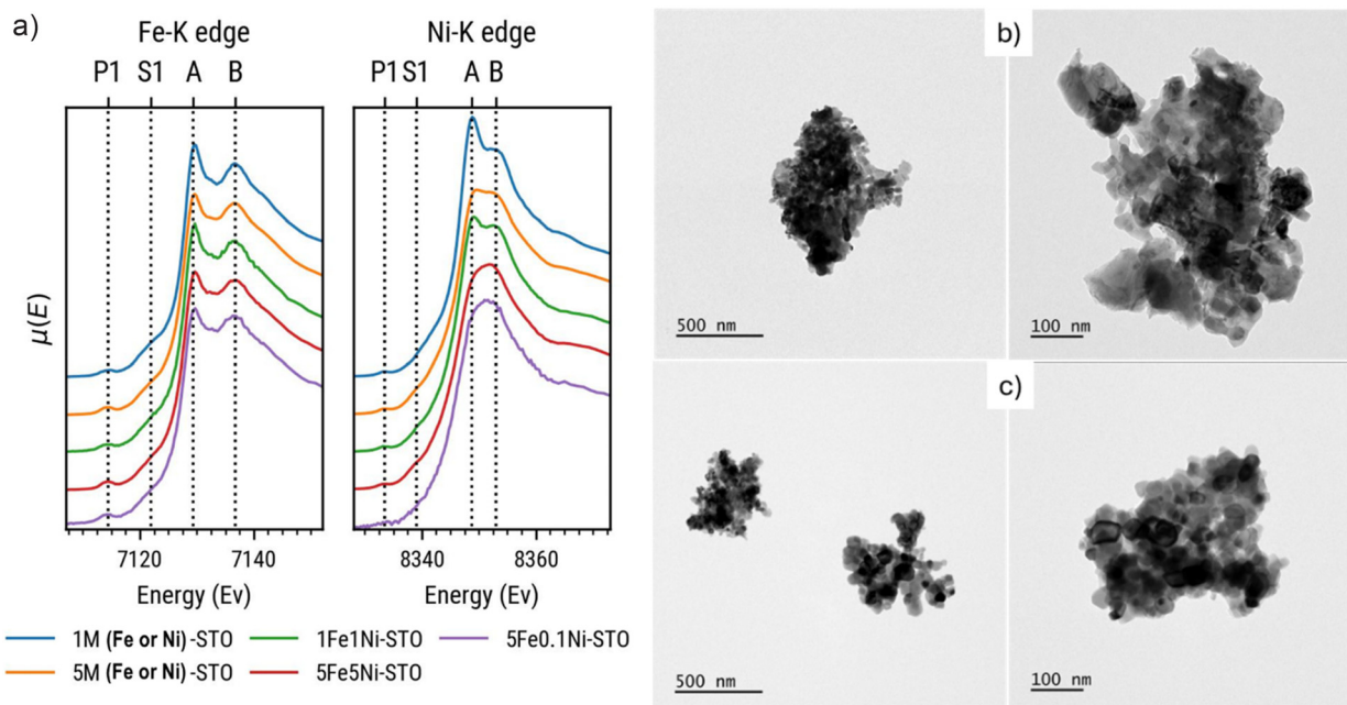
Fig. 2 (a) XAS spectra of all the as-prepared doped and co-doped perovskite samples; (b and c) representative TEM images of the 5Fe-STO and 5Fe5Ni-STO parental structures.
