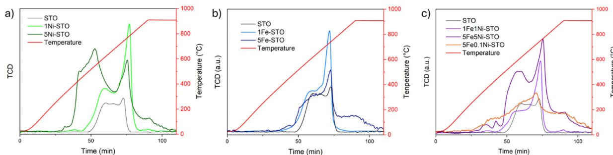
Fig. 3 TPR profiles of (a) Ni-doped and (b) Fe-doped and (c) Fe-Ni co-doped perovskites powders. The behavior of undoped ST0 sample is reported for comparison.
