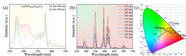
Fig. 3 (a) PLE spectra of Tb^{3+} ions (548 nm) and Eu^{3+} ions (596 nm). (b) PL spectra of Cs_2NaTb_{0.95}Eu_{0.05}Cl_6 under various excitation wavelengths. (c) CIE coordinates of the Cs_2NaTb_{0.95}Eu_{0.05}Cl_6 emission.
