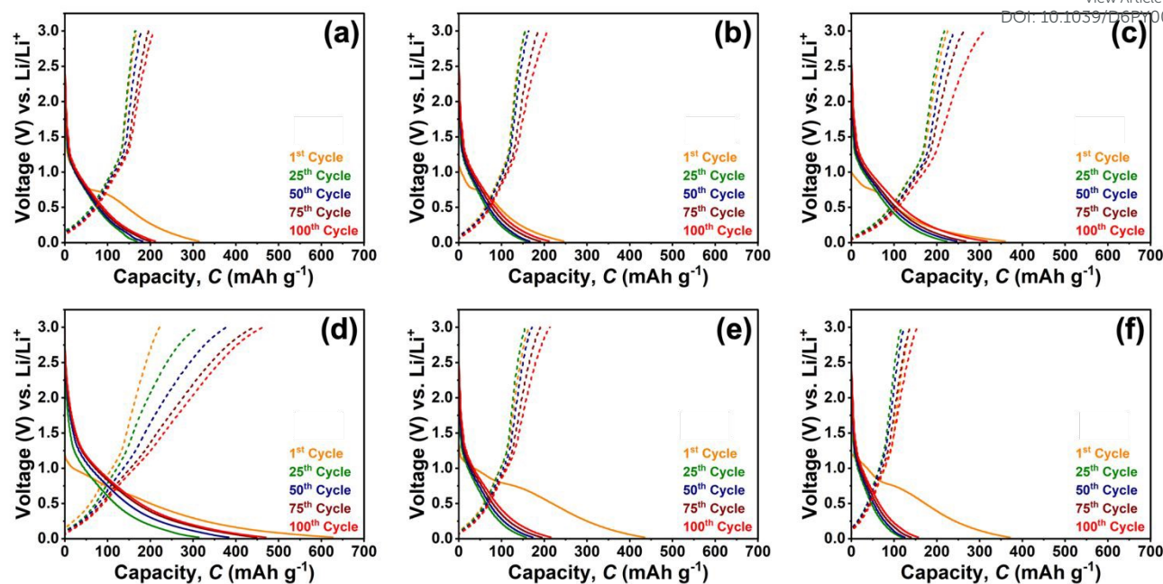
Figure 2. Galvanostatic charge-discharge profiles of (a) PQ-a, (b) PQ-b, (c) PQ-c, (d) PQ-d, (e) PQ-e, and (f) PQ-f measured at 0.1 \text{ A g}^{-1} within a voltage range of 0.02\text{--}3.0 \text{ V} (vs. \text{Li/Li}^+ ).
