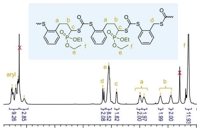
Fig. 5 ^1\text{H} NMR spectrum of \text{p}(\text{DEVP}_{0.4}\text{-BOT}_{0.6})_n (Table 1, entry 8).
