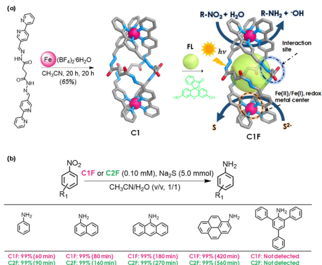
Fig. 7 (a) Schematic representation of self-assembly of C1 and the photocatalytic system of C1F for the combination of H 2 S splitting and hydrogenation of nitroaromatics. (b) Photocatalytic reduction of different nitroaromatics into aminoarenes under standard conditions: substrate (0.50 mmol).
