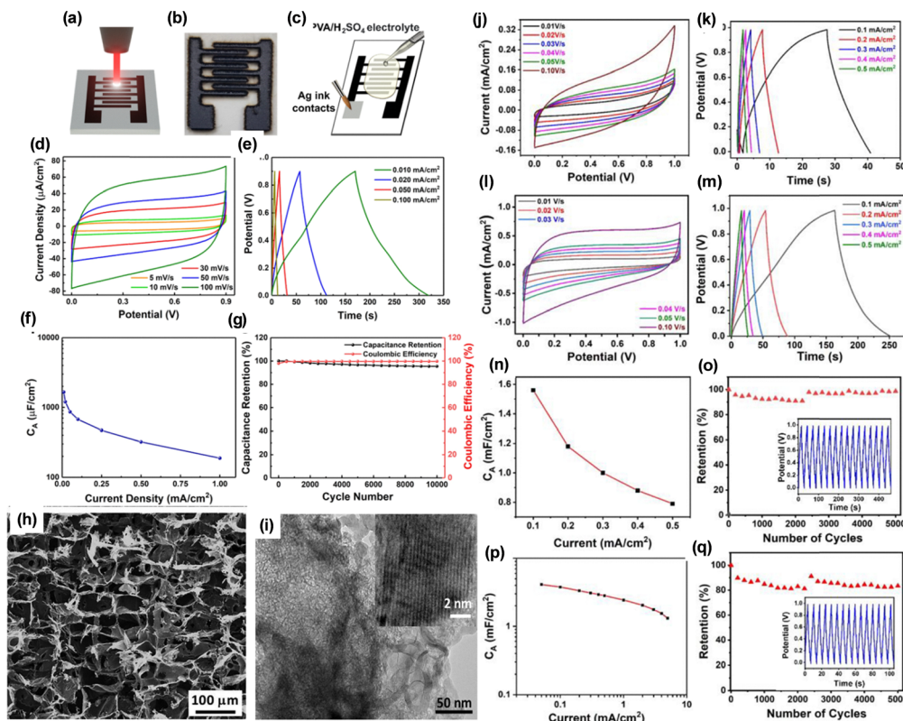
Fig. 5 (a) Illustration of the direct laser writing process used to fabricate micro-supercapacitor (MSC) electrodes or laser induced graphene (LIG); (b) LIG-MSC electrodes patterned directly onto a parylene-C substrate; (c) schematic showing the structural assembly of the LIG-MSC device; (d) CV curves demonstrating electrochemical behavior; (e) charge-discharge profiles at various current densities; (f) specific capacitance values as a function of current density; and (g) long-term cycling stability and Coulombic efficiency at 0.5 \text{ mA cm}^{-2} for the LIG-MSCs fabricated on parylene-C. Reproduced with permission. 136 (h) SEM image of image of the LIG graphitized area, (i) TEM image of LIG. (j) CV of a representative open LIG device, (k) GCD curves of open LIG device (l) CV of a sandwich LIG device (m) GCD curves of sandwich LIG device. (n) Plot of area capacitance ( C_A ) vs. current density for open LIG device and corresponding (o) cycling stability over 5000 cycles. (p) Plot of area capacitance ( C_A ) vs. current density for sandwich LIG device and corresponding (q) cycling stability over 5000 cycles. Reproduced with permission. 135
