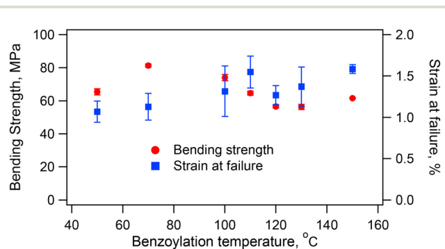
Fig. 5 Plot of bending strengths and strains at failure of benzyated composites against benzylation temperatures. The standard errors obtained from three to four measurements were represented by error bars.
