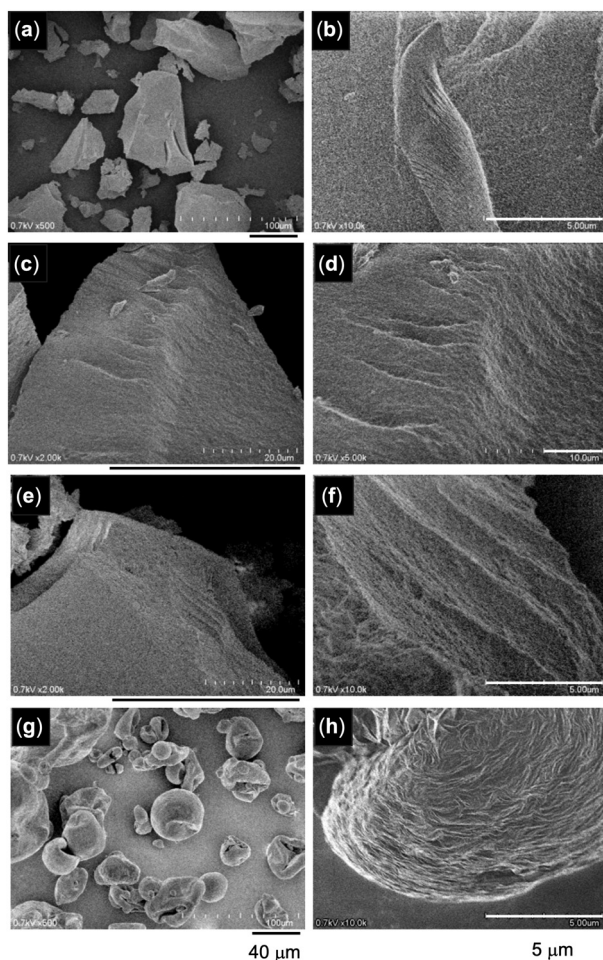
Fig. 9 FE-SEM images of (a and b) L -PAAm-DSBP composites, (c and d) M -PAAm-DSBP composites, (e and f) H -PAAm-DSBP composites and (g and h) DSBP. Black scale bars: 40 \mu m; white scale bars: 5 \mu m.
