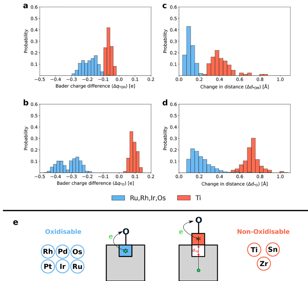
Fig. 3 Probability distributions of the Bader charge difference ( \Delta q_A ) at the adsorption site atom in the RuRhIrOsTi high entropy oxides dataset after (a) *OH, and (b) *O adsorption. (c) Probability distributions of the change in the distance ( \Delta d_A ) between the adsorption site atom and the oxygen atom underneath after *OH and (d) *O adsorption. Data for Ru, Rh, Ir, and Os adsorption sites are aggregated into a single distribution for comparison with the distribution based on data for Ti sites. (e) Schematic figure of the proposed explanation for the different adsorption energies trends observed for Ti, Sn, and Zr guests and Ru, Rh, Ir, Os, Pd, and Pt guests.
