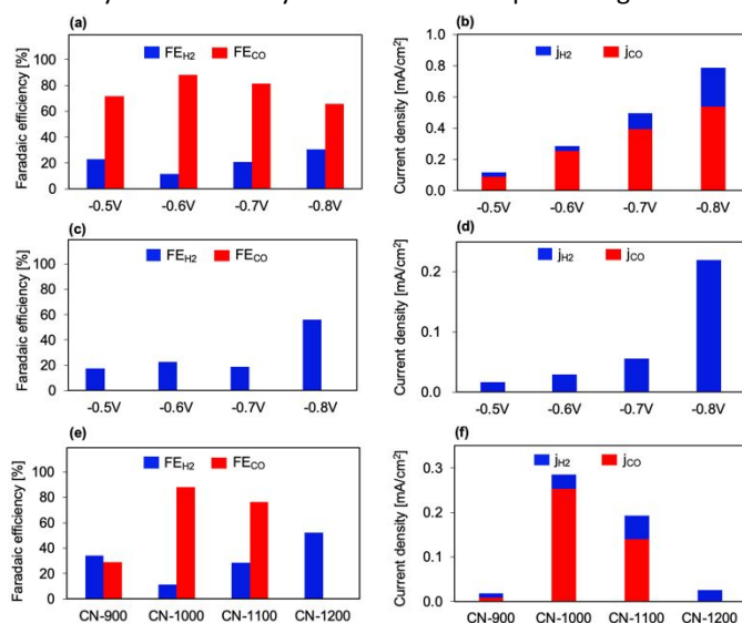
Fig. 2 (a) Faradaic efficiencies of CO and H 2 using CN-1000 within the potential window from -0.5 V to -0.8 V vs. RHE in CO 2 -saturated 0.1 M KHCO 3 solution, (b) the comparison of partial current density of CO and H 2 using CN-1000, (c) faradaic efficiencies of CO and H 2 using C-1000 within the potential window from -0.5 V to -0.8 V vs. RHE in CO 2 -saturated 0.1 M KHCO 3 solution, (d) the comparison of partial current density of CO and H 2 using C-1000, (e) faradaic efficiencies of CO and H 2 using CN-T within the potential window at -0.6 V vs. RHE in CO 2 -saturated 0.1 M KHCO 3 solution and (f) the comparison of partial current density of CO and H 2 using CN-T.
