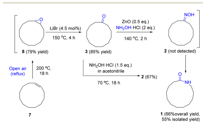
Fig. 2 Result for the sequential one-pot reaction to achieve either laulolactam 1 or cyclododecanone oxime 2 from cyclododecene 7 .
