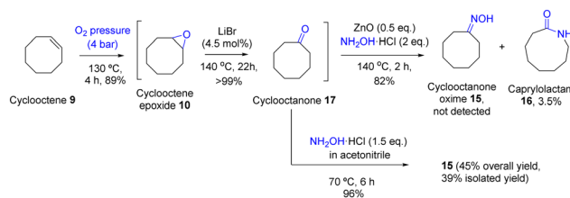
Fig. 3 Result for the sequential one-pot reaction to achieve cyclooctanone oxime 15 or caprylactam 16 from cyclooctene 9 . All yield results refer to gas chromatography (GC) yields, checked also by mass spectrometry (GC-MS) and using dodecane as an external standard.
