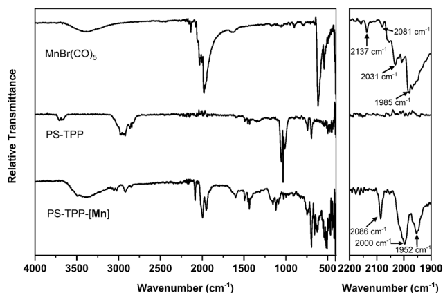
Fig. 1 ATR-FTIR analysis for \text{MnBr}(\text{CO})_5 (top), PS-TPP (centre) and PS-TTP-[Mn] (bottom). The right-hand panel shows an expansion of the region between 2200 and 1900 \text{cm}^{-1} .
