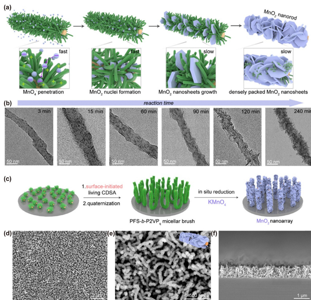
Fig. 14 (a) Schematic illustration of the formation of nanorods densely coated with thin \text{MnO}_2 nanosheets via a direct redox reaction between PFS- b -P2VP q cylindrical micelles and \text{KMnO}_4 . (b) TEM images depicting the progressive deposition and growth of manganese oxide on PFS- b -P2VP q cylindrical micelles during the redox process. (c) Schematic representation of \text{MnO}_2 nanoarray fabrication, involving surface-initiated living growth of PFS- b -P2VP q micellar brushes followed by an in situ redox reaction with \text{KMnO}_4 under ambient conditions. (d, e) Top-view and (f) cross-sectional SEM images of the \text{MnO}_2 nanoarray on a silicon wafer. Reproduced from ref. 92 with permission from American Chemical Society, copyright 2025.
