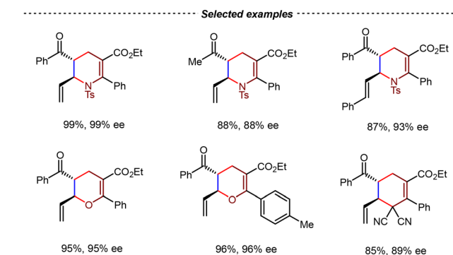
Scheme 48 Pd(0)-catalyzed asymmetric cross inverse-electron-demand [4+2] cycloadditions between 2,4-dienyl carbonyls and 1-heterodienes/allylidenemalononitriles.
