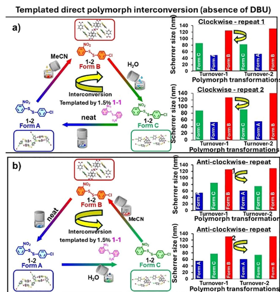
Fig. 35 Three-polymorph interconversion of 1-2 under ball milling. ≥1.5 mol% 1-1 enables transformations, likely acting as a template. (a) Clockwise: Form B → Form C → Form A → Form B → Form C → Form A → Form B. (b) Anticlockwise: Form B → Form A → Form C → Form B → Form A → Form C. Form A forms by NG; Form C by LAG with water; Form B by LAG with MeCN. Crystallite sizes: Form A = 40–60 nm; Form C = 70–90 nm; Form B = 120–140 nm. 60 Adapted from ref. 60 with permission from The Royal Society of Chemistry.
