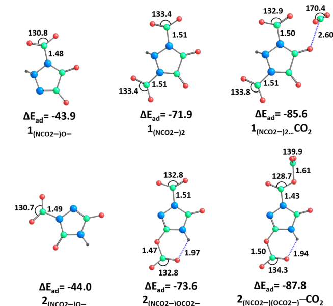
Fig. 8 Optimized structures of CO 2 adduct with dianions at the M06-2X/cc-pVQZ level of theory. Distances in Å, angles in degrees and \Delta E_{\text{ad}} in kcal mol −1 . Color key: gray – H, blue – N, green – C, red – O.
