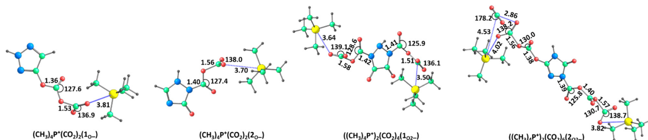
Fig. 10 Representative structures of triazolate- \text{CO}_2 adducts in ethanol with tetramethylphosphonium counter-ions, computed at the M06-2X/SMD/cc-pVTZ level. Distances in Å, angles in degrees; Color key: gray – H, blue – N, green – C, red – O, yellow – P.
