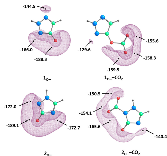
Fig. 5 MESP topography of anions 1O - , 2O - and their most stable \text{CO}_2 adducts computed at the M06-2X/cc-pVQZ level of theory. Black dots indicate V_{\min} value in \text{kcal mol}^{-1} . Isosurface value: -125 \text{ kcal mol}^{-1} . Color key: gray – H, blue – N, green – C, red – O.
