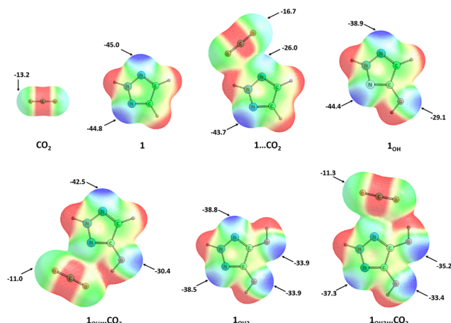
Fig. 3 MESP on the 0.005 a.u. isodensity surface for \text{CO}_2 , 1 , 1OH , 1OH 2 , and their \text{CO}_2 complexes. V_{\min} values ( \text{kcal mol}^{-1} ) and \text{N}\cdots\text{C} , \text{O}-\text{H}\cdots\text{O} distances (Å) at the M06-2X/cc-pVQZ level of theory. Color gradient: blue (electron-rich) to red (electron-deficient).
