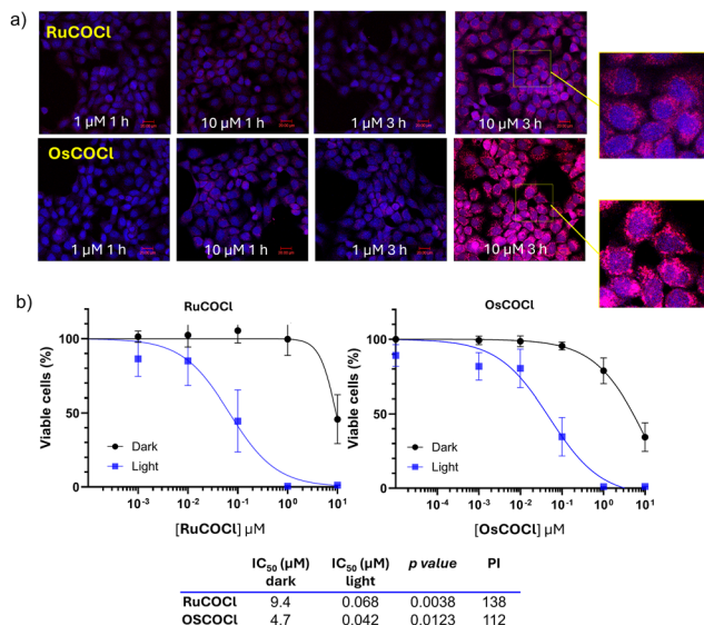
Fig. 2 (a) Time and dose-dependent cellular uptake of RuCOCl and OsCOCl (1–10 μM) in A431 cells by CLSM. DAPI was used to counterstain nuclei ( \lambda_{\text{exc}} = 405 nm, \lambda_{\text{em}} = 461 nm), complex fluorescence appears in purple-red ( \lambda_{\text{exc}} = 405 nm, \lambda_{\text{em}} = 600 –640 nm). Confocal fluorescence images; scale bar = 20 μm. Magnified insets are provided for the 10 μM, 3 h incubation conditions for both RuCOCl and OsCOCl . (b) Cell viability by MTT assay in the dark or upon photoactivation ( \lambda_{\text{max}} = 462 nm, 160 mW): absorbance was normalized to untreated controls; dose–response curves were fitted by nonlinear regression and IC 50 values compared using the extra sum-of-squares F test ( n = 3 ).
