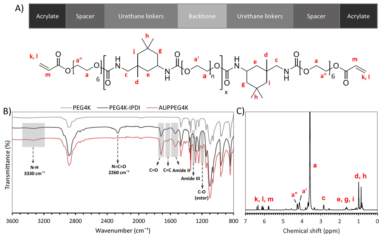
Fig. 1 Structure of the acrylate-terminated, urethane-based PEG polymer (AUP) ( n depends on the molar mass of the backbone, x = 1-3 ). (A) Molecular structure of the AUP. (B) FTIR spectra of the starting PEG, the intermediate product (PEG-IPDI) and the final AUP. (C) ^1\text{H} -NMR spectrum of the AUP. In (B) and (C), the 4000 \text{ g mol}^{-1} PEG derivative is shown (indicated as AUPPEG4K).
