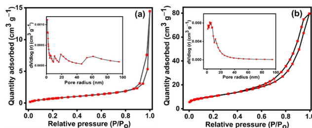
Fig. 7 \text{N}_2 adsorption-desorption BET isotherms with corresponding BJH pore-size distributions plots (insets): (a) \text{NiMoO}_4 and (b) \text{NiMoO}_4/\text{C} (D50).
