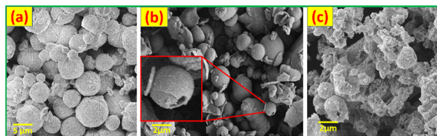
Fig. 5 FESEM images of (a) \text{NiMoO}_4 , (b) CNS and (c) \text{NiMoO}_4/\text{C} (D50).
