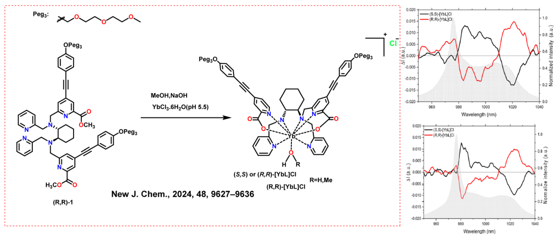
Scheme 41 (Left) Chemical structures of the ligands and Ln complexes (R,R)/(S,S)\text{-[Yb]Cl} . 91 (Right) CPL spectra of (S,S)\text{-[Yb]Cl} and (R,R)\text{-[Yb]Cl} complexes in water (up) and in methanol (bottom) emitting in the near-infrared region. Reproduced from ref. 91 with permission from the Royal Society of Chemistry, copyright [2024]. 91
