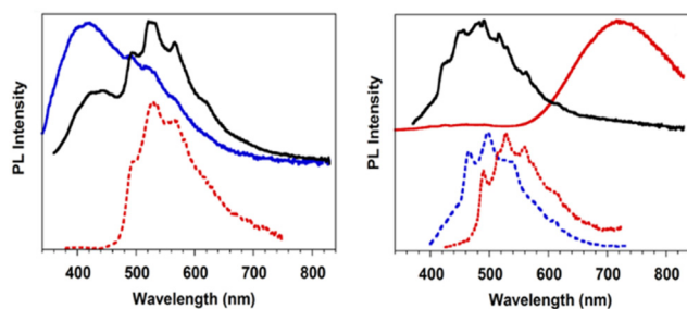
Fig. 16 Left: Emission spectra of TT-DITFB at 298 K: top: PL at \lambda_{exc} = 300 nm (blue) and \lambda_{exc} = 350 nm (black); bottom: phosphorescence ( \lambda_{exc} = 350 nm, delay 0.5 ms, window 1 ms, red dashed); right: emission spectra of TT-DITFB crystals at 77 K: top: PL at \lambda_{exc} = 340 nm (black), \lambda_{exc} = 300 nm (red); bottom: phosphorescence at \lambda_{exc} = 320 nm (delay 10 ms, window 50 ms, blue dashed) and \lambda_{exc} = 370 nm (delay 10 ms, window 50 ms, red dotted). Adapted with permission from ref. 71. Copyright 2019, John Wiley and Sons.
