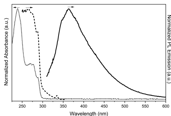
Fig. 17 Absorption (dotted line), excitation (dashed line, \lambda_{em} : 374 nm) and PL emission (continuous line, \lambda_{exc} : 290 nm) spectra of TT-CCH in DCM.
