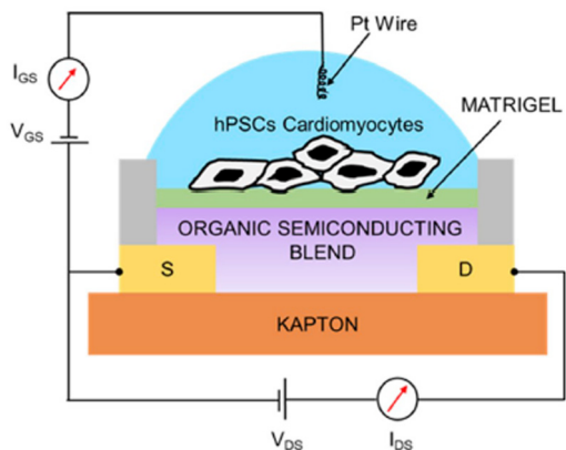
Fig. 64 Schematic diagram of the EGOFET coupled to hPSCs-CMs grown as a cluster of cells (reproduced with permission from ref. 235. Copyright 2020, Elsevier).
