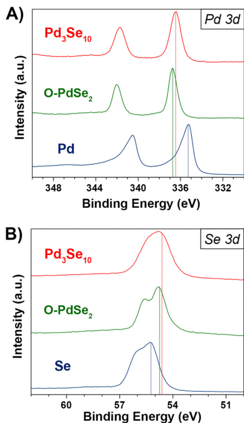
Fig. 4 (A) Pd 3d XPS spectra for \text{Pd}_3\text{Se}_{10} , \text{O-PdSe}_2 , and palladium powders. (B) Se 3d XPS spectra for \text{Pd}_3\text{Se}_{10} , \text{O-PdSe}_2 , and selenium powders.
