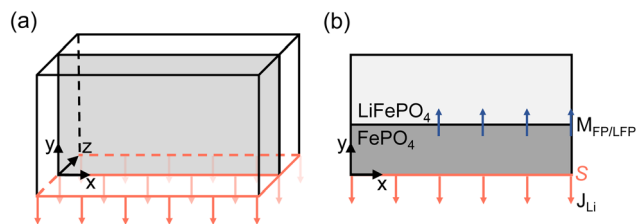
Fig. 3 Schematics showing (a) a three dimensional system of bulk LiFePO 4 , and (b) a cross-section of the two-dimensional setup showing the direction of the Li charge transfer rate ( J_{\text{Li}} ) perpendicular to surface S and the FP/LFP interface moving in the opposite direction ( M_{\text{FP/LFP}} ).
