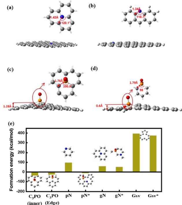
Fig. 6 (a) Optimized models for graphitic N doped graphene. (b) Optimized models for pyridinic N doped graphene. (c) Optimized models for C 3 PO doped graphene. (d) Optimized models for C 2 PO 2 doped graphene. (e) The formation energy of the various structures. * represents the generation energy of the structure in the presence of C 3 PO.
