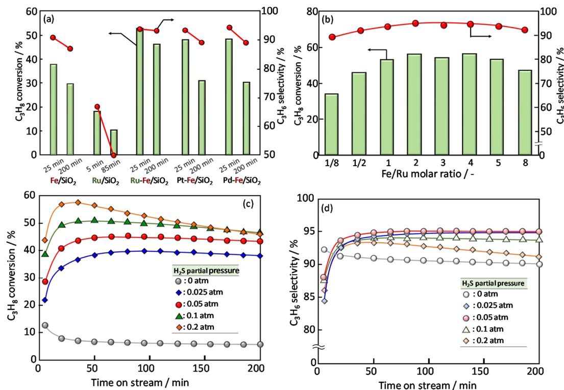
Fig. 1 (a) Effect of noble metal (Ru, Pt, Pd) loading onto \text{Fe}/\text{SiO}_2 for propane dehydrogenation with \text{H}_2\text{S} co-feeding. (b) Optimum ratio of Fe to Ru in \text{Ru}-\text{Fe}/\text{SiO}_2 catalyst. (c) Propane conversion and (d) propylene selectivity over \text{Ru}-\text{Fe}/\text{SiO}_2 catalyst under various \text{H}_2\text{S} partial pressures.
