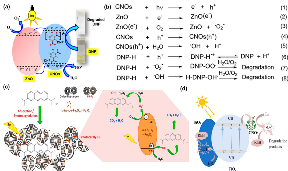
Fig. 11 (a) An illustration of the photodegradation of DNP by the T-ZnO-CNO hybrid composite, (b) a plausible mechanism of the photocatalytic degradation of DNP by the T-ZnO-CNO hybrid composite under visible-light irradiation, 85 (c) visual depiction of the synergistic adsorption-photocatalytic processes driving methylene blue degradation by the engineered PR-Fc catalyst, 107 (d) the mechanism diagram of \text{SiO}_2/\text{CNOs}/\text{TiO}_2 in the degradation of dyes in visible light. 81
