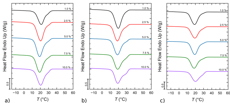
Fig. 1 DSC cooling curves at 20\text{ °C min}^{-1} of PCL composites with (a) NdFeB, (b) SFO, and (c) SFO-CFO magnetic micro- and nanoparticles in the composition range of 1–10%.
