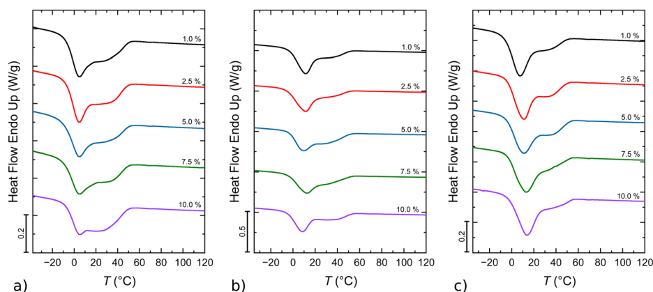
Fig. 2 DSC cooling curves at 20\text{ °C min}^{-1} of PBSA composites with (a) NdFeB, (b) SFO, and (c) SFO-CFO magnetic micro- and nanoparticles in the composition range of 1–10%.
