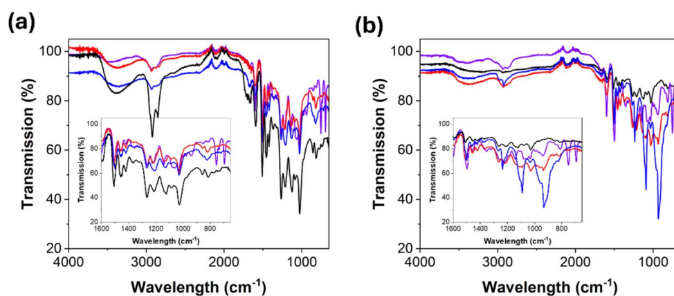
Fig. 5 FTIR spectra of unmodified (a) SL (black), SL-BZ-aniline (purple), SL-BZ-A (red) and SL-BZ-B (blue) and (b) KL (black), KL-BZ-aniline (purple), KL-BZ-A (red) and KL-BZ-B (blue).
