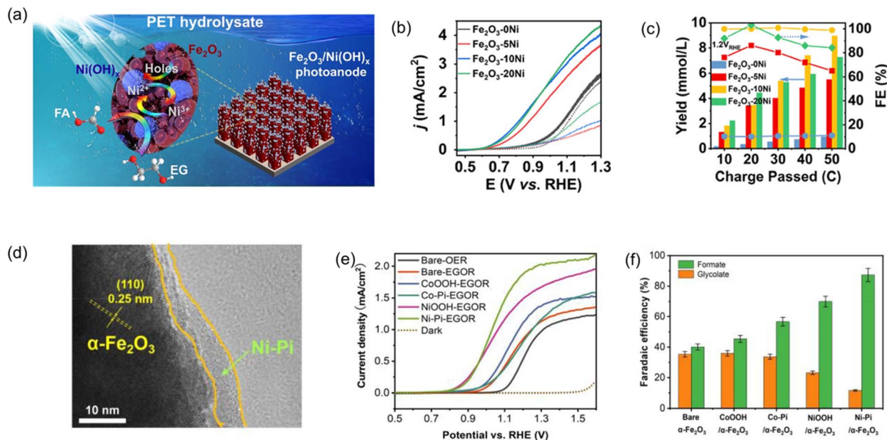
Fig. 12 (a) Schematic of the surface modification of the Fe 2 O 3 photoanode with Ni(OH) x for selective oxidation of EG into FA. Enhancement of (b) photocurrent and (c) the yield and FE of FA with the charge passed using Fe 2 O 3 /Ni(OH) x photoanodes modified with different concentrations of Ni(OH) x . Reproduced with permission. 118 Copyright 2022, American Chemical Society. (d) TEM image of the Ni-Pi/α-Fe 2 O 3 photoanode. (e) LSV curves and (f) FE for α-Fe 2 O 3 with different co-catalysts. FE was derived at 1.1 V for 2 h. Reproduced with permission. 9 Copyright 2023, Elsevier.
